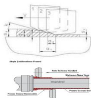
Flowforming
